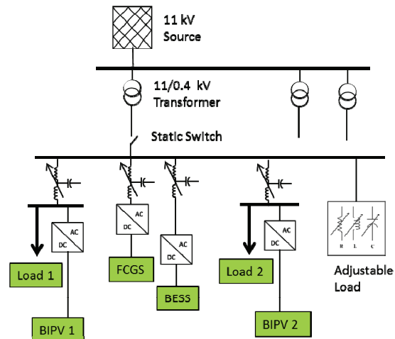
Figure 2. Proposed Microgrid architecture
