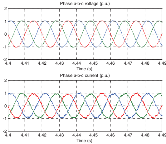
Figure 6. PVGS output voltage and current
