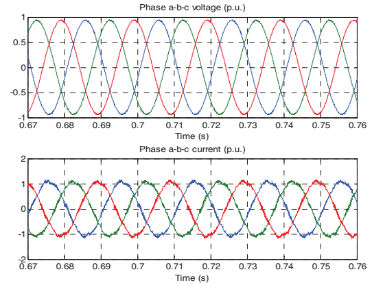
Figure 8. BESS output voltage and current
