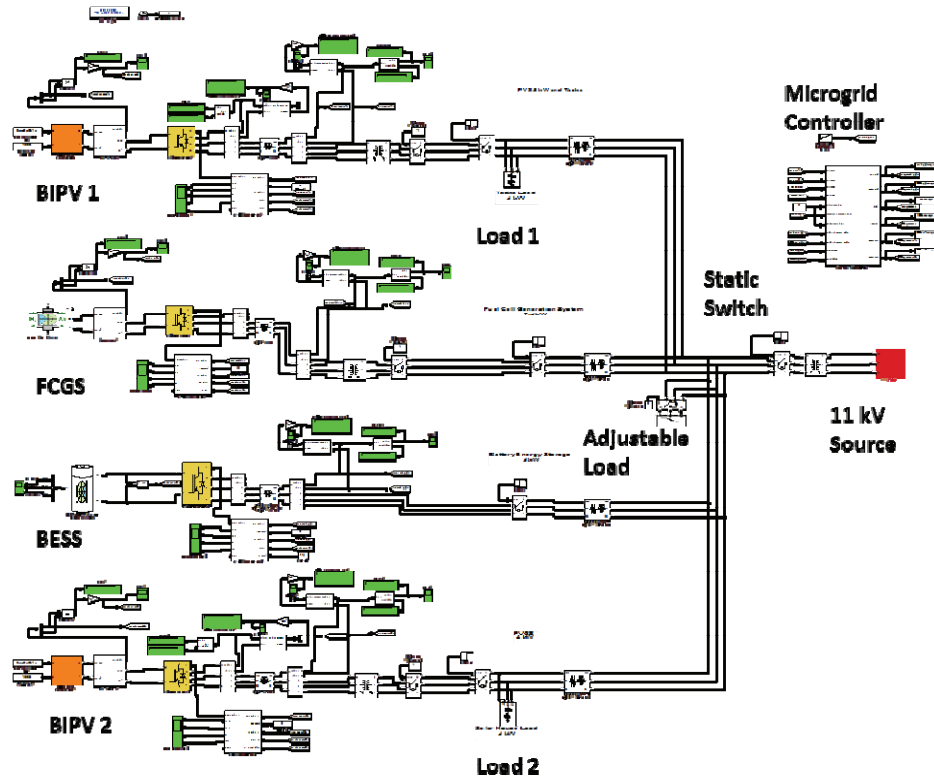
Figure 5. Snapshot of Microgrid model in SimPowerSystems
